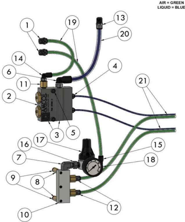
T60A-2B-1AX-NAR15 Complete Assembly
